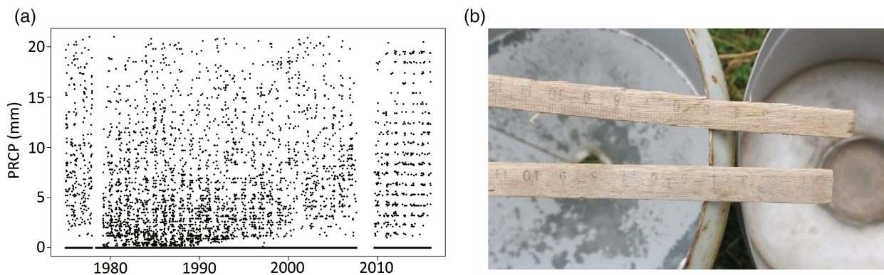
Figure 4. (a) In the data of the Bolivian station Choroco, precipitation (PRCP) values between 0 and up to about 3 mm are largely missing until the early 1980s and from the 1990s onward. Values >21 mm are not shown in the plot. (b) Precipitation in Bolivia is measured by sticking a scale in the inner container of the Hellmann rain gauge and reading the water mark on the scale (1 cm on the scale corresponds to 1 mm of PRCP). Some scales are aged and have faded scale marks, especially towards the ends. [Colour figure can be viewed at wileyonlinelibrary.com ].
